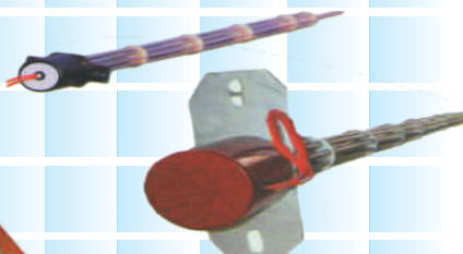
Corrugation Machine Heater
