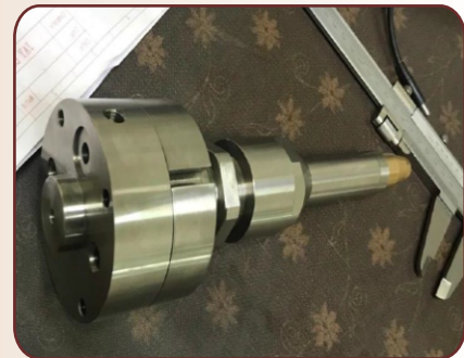
SS Water Cooling Blow Pin with Belgian Copper Tip
